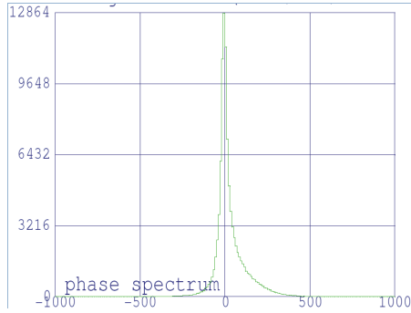
Figure 3: Bunch length after the drift space of 34 cm beyond the Prebuncher .
