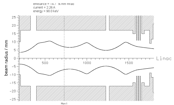
Figure 5: Simulation of a 2 A beam propagating through the beam guiding elements based on the paraxial equations.
