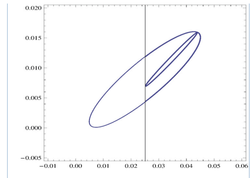
Figure 7: Shown is the acceptance ellipse of the synchrotron at the injection point, the phase space ellipse of the beam and the edge of the injection septum.
