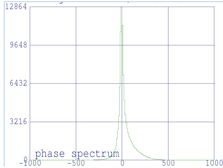
Figure 3: Bunch length after the drift space of 34 cm beyond the Prebuncher .
