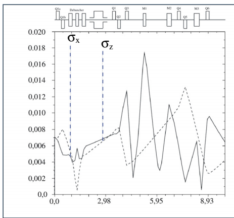
Figure 6: MAD simulation of the transverse beam dynamics of the transfer line. Shown are the horizontal and vertical beam width \sigma_x and \sigma_z versus the position in the transfer line.
