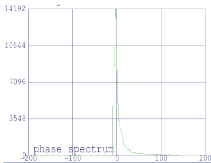
Figure 4: bunch length after the travelling wave buncher. Shown is the number of particles versus the phase position of the particles relative to the main particle.
